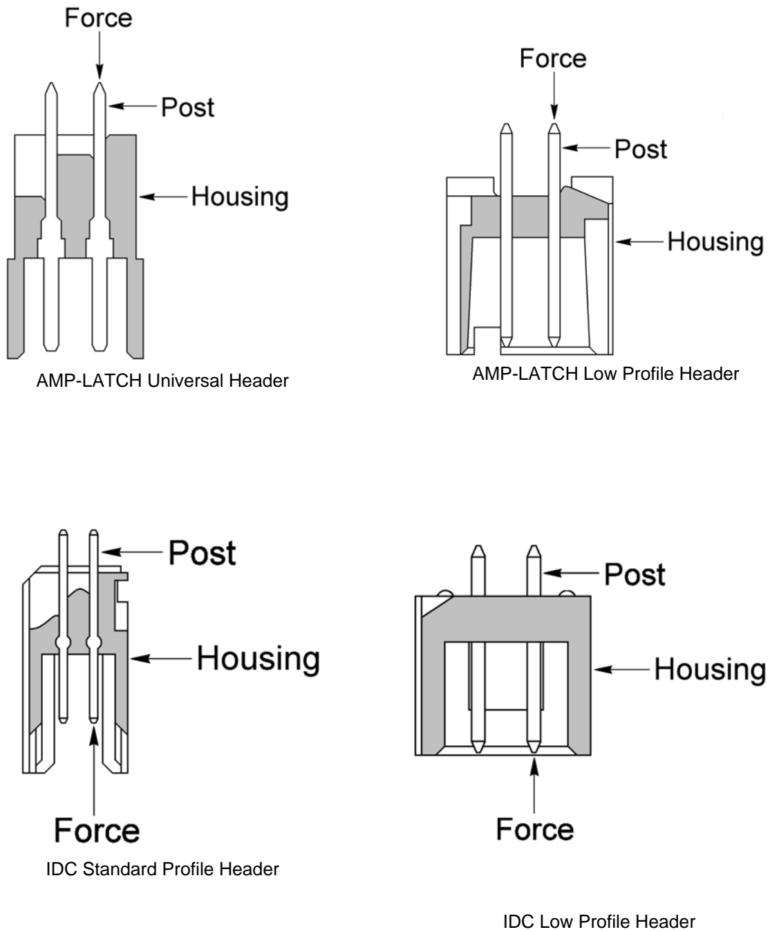
Figure 3 Contact Retention
