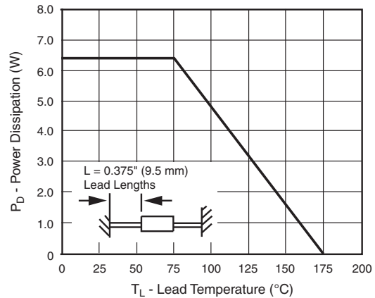
Fig. 8 - Power Derating Curve
