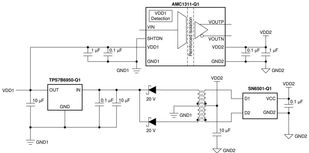
Figure 52. SN6501-Q1-Based, High-Side Power Supply
