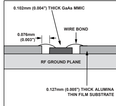
Figure 36. Die Without the Moly Tab
