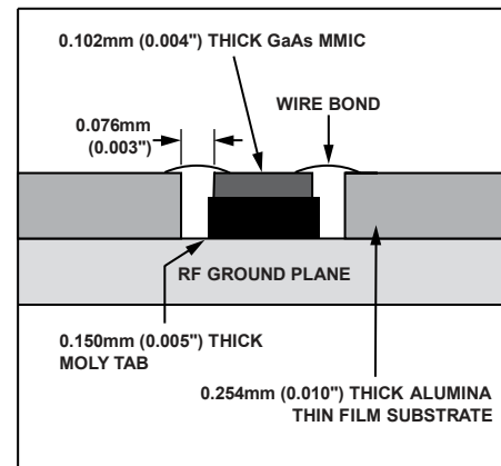
Figure 37. Die With the Moly Tab
