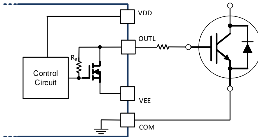
Figure 38. Active Pulldown
