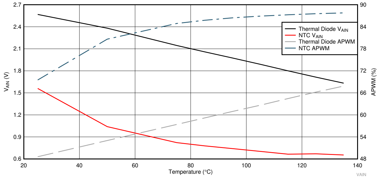
Figure 55. Thermal diode and NTC V_{AIN} and Corresponding Duty Cycle at APWM
