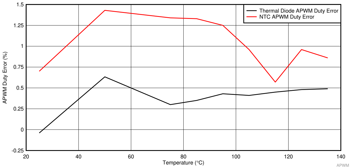
Figure 56. APWM Duty Error Without Calibration
