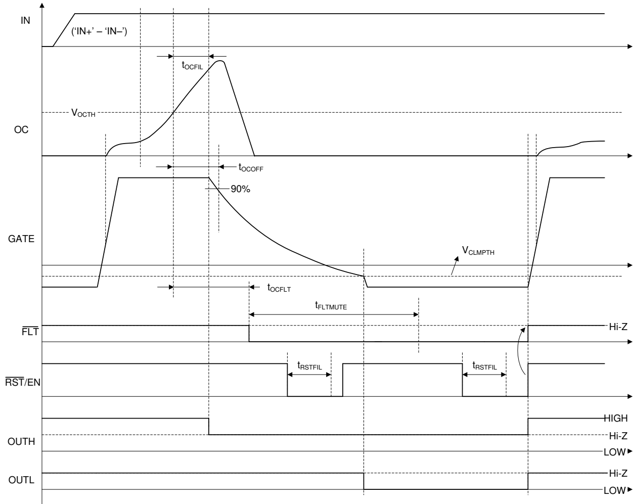
Figure 36. OC Protection with Soft Turn-OFF
