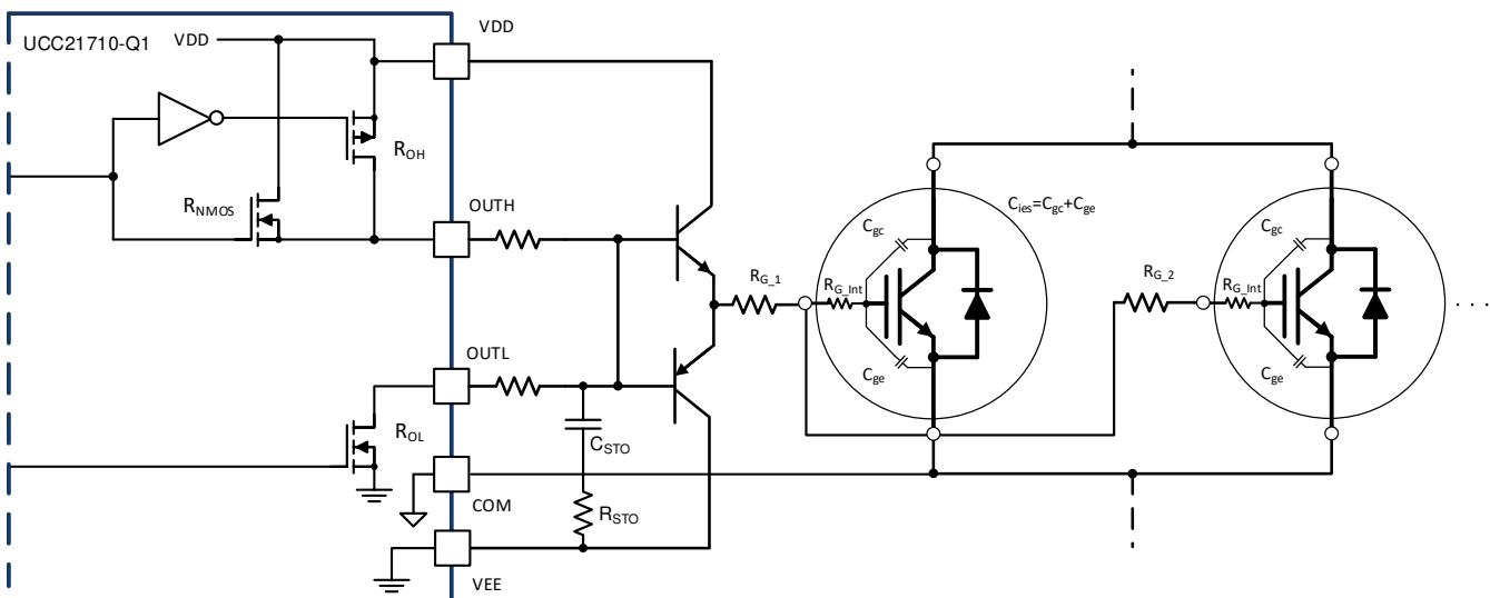
Figure 59. Current Buffer for Increased Drive Strength
