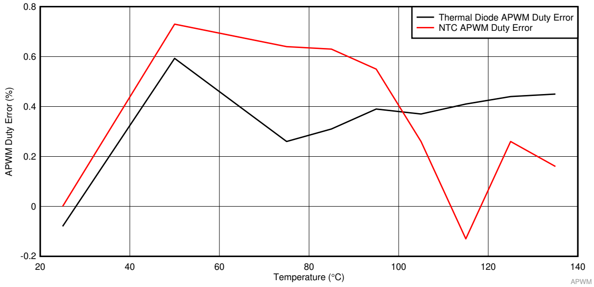
Figure 57. APWM Duty Error with Single-Point Calibration
