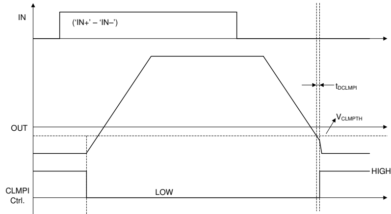
Figure 33. Timing Diagram for Internal Active Miller Clamp Function
