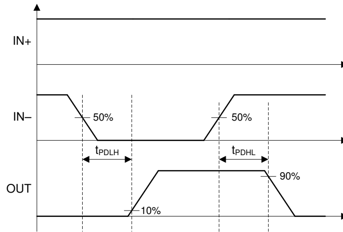
Figure 28. Inverting Logic Propagation Delay Measurement
