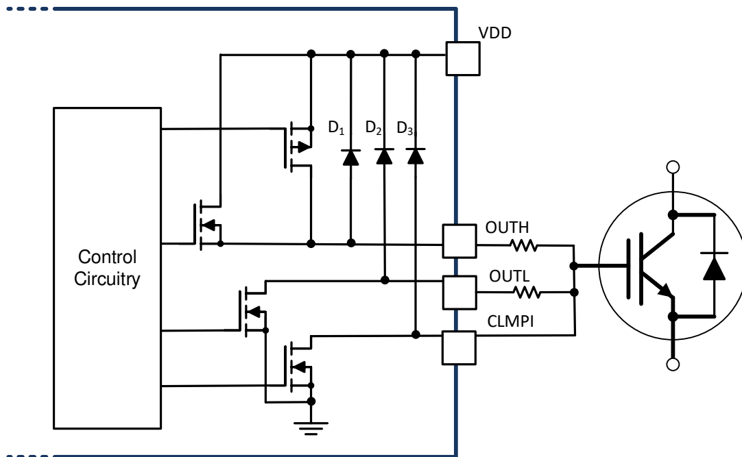
Figure 39. Short Circuit Clamping
