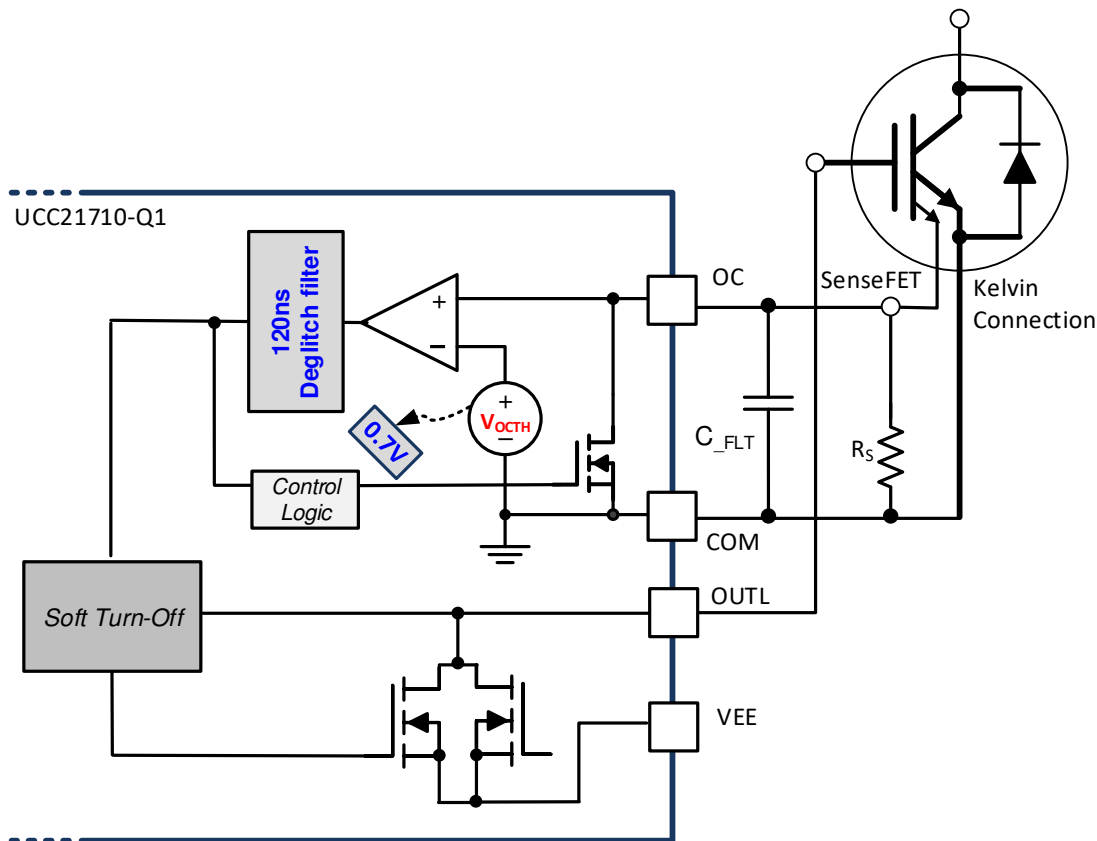
Figure 42. Soft Turn-off
