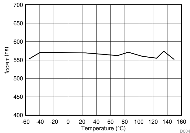
Figure 26. t_{OCFLT} OC to \overline{FLT} Low Delay Time vs. Temperature
