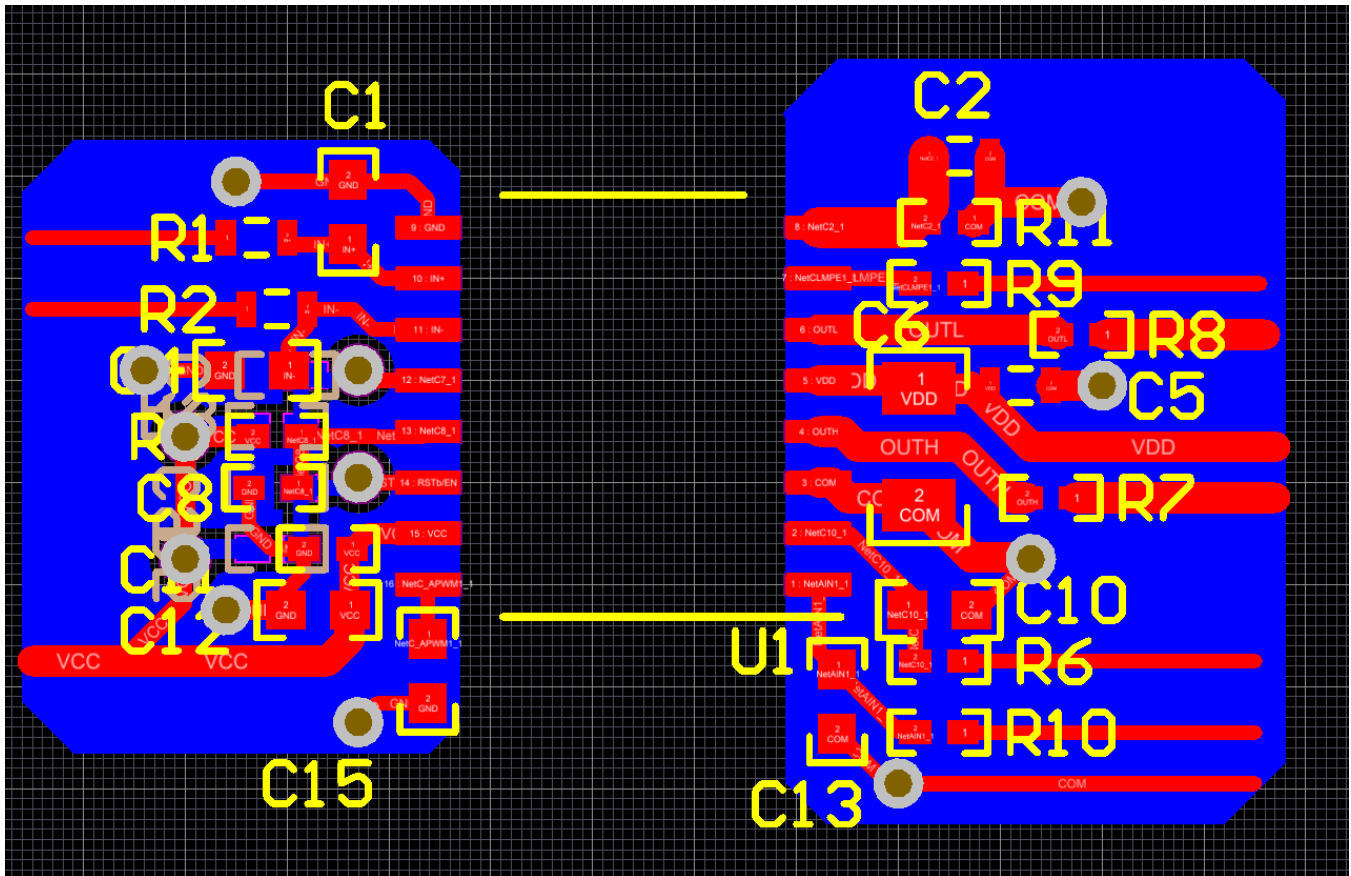
Figure 60. Layout Example
