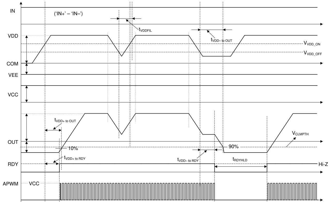
Figure 35. VDD UVLO Protection Timing Diagram
