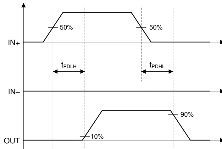
Figure 27. Non-inverting Logic Propagation Delay Measurement
