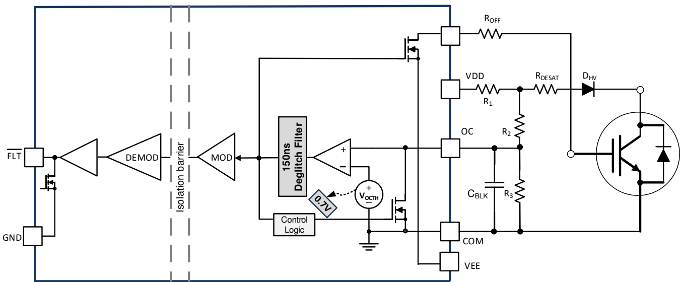
Figure 51. Overcurrent and Short Circuit Protection Based on Desaturation Circuit
