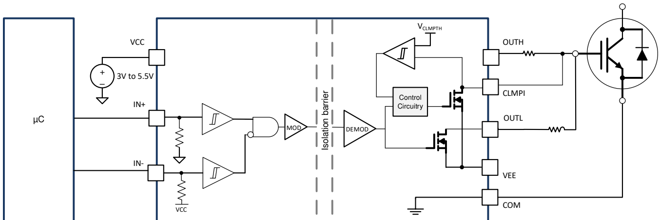
Figure 40. Active Miller Clamp
