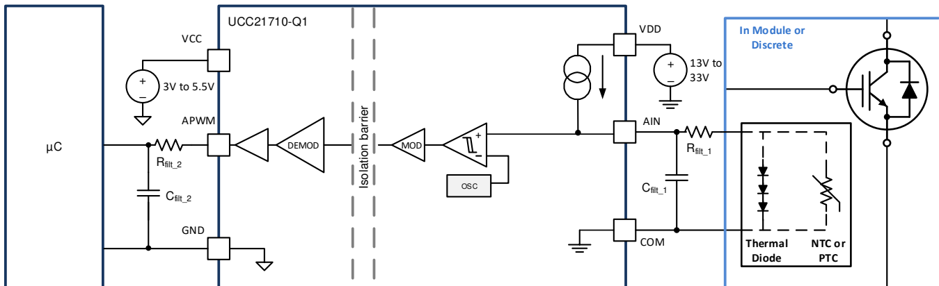
Figure 54. APWM Channel with Filtered Output
