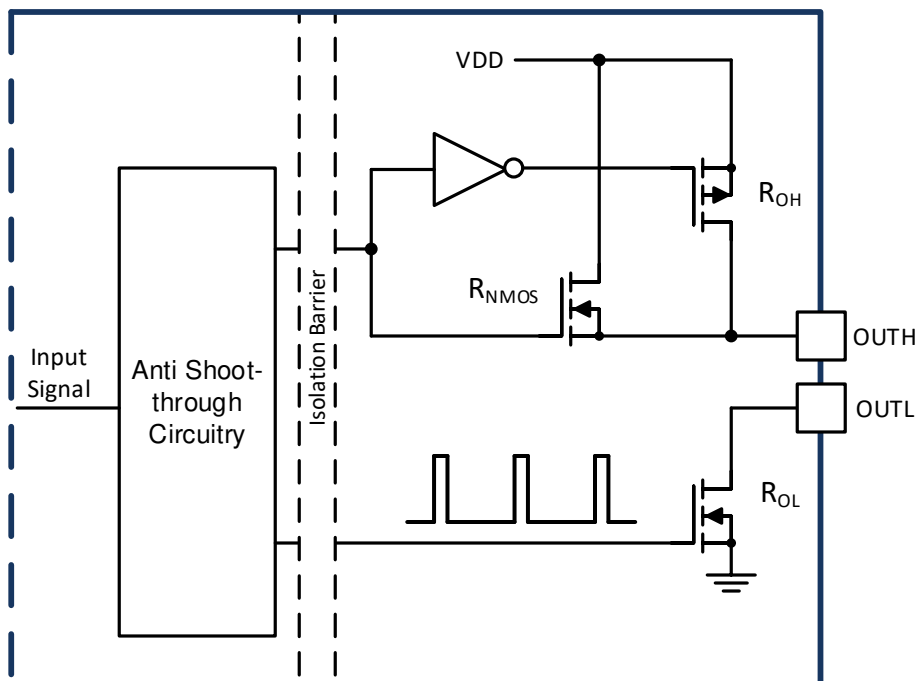
Figure 37. Gate Driver Output Stage
