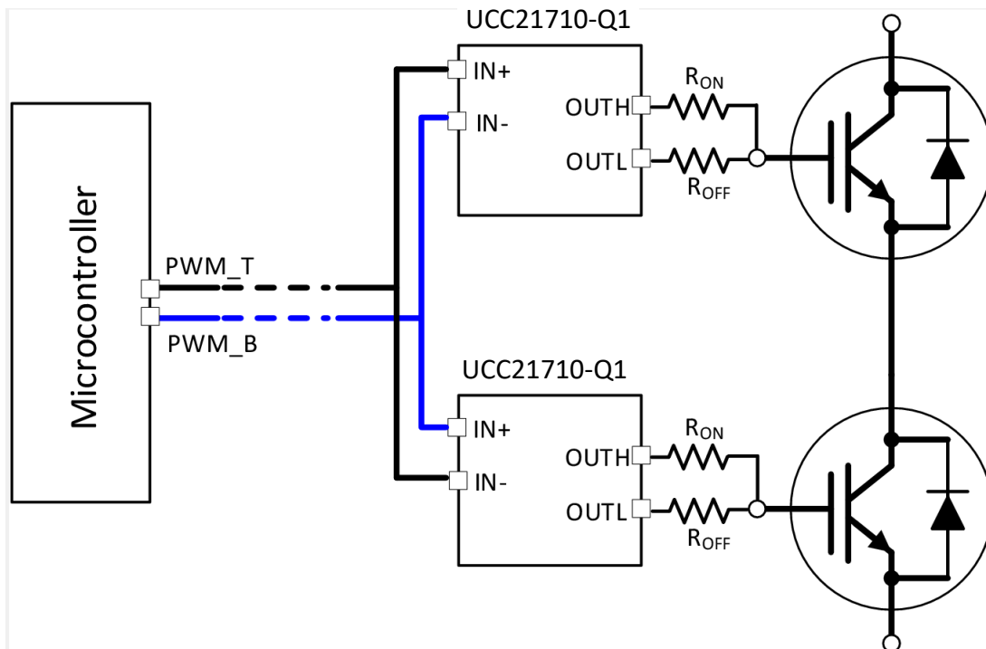
Figure 45. PWM Interlock for a Half Bridge
