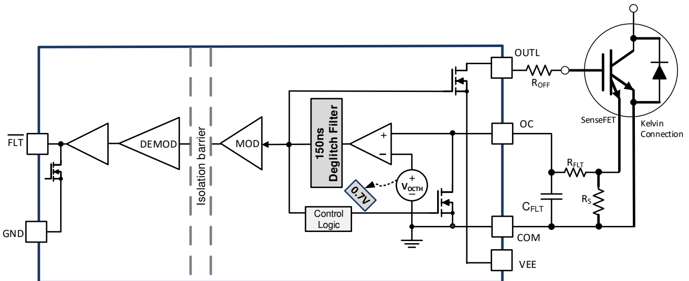
Figure 50. Overcurrent and Short Circuit Protection Based on IGBT Module with SenseFET
