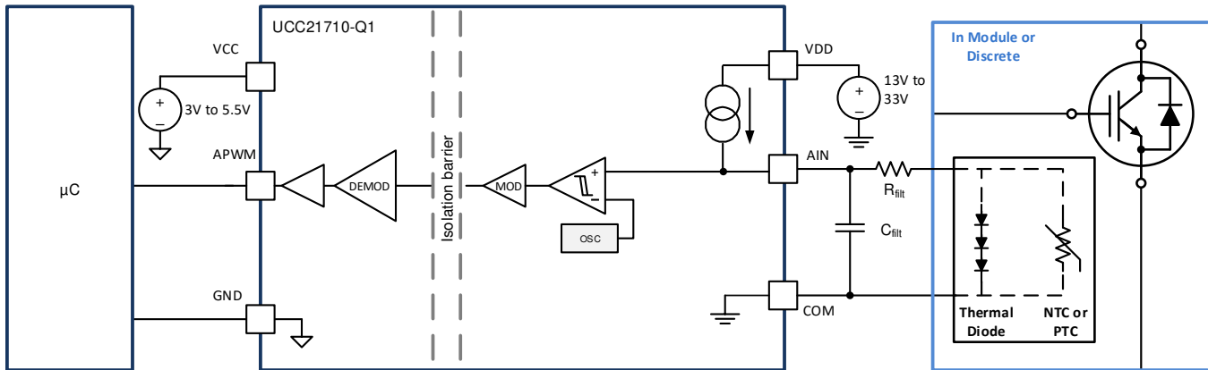
Figure 53. Thermal Diode or Thermistor Temperature Sensing Configuration
