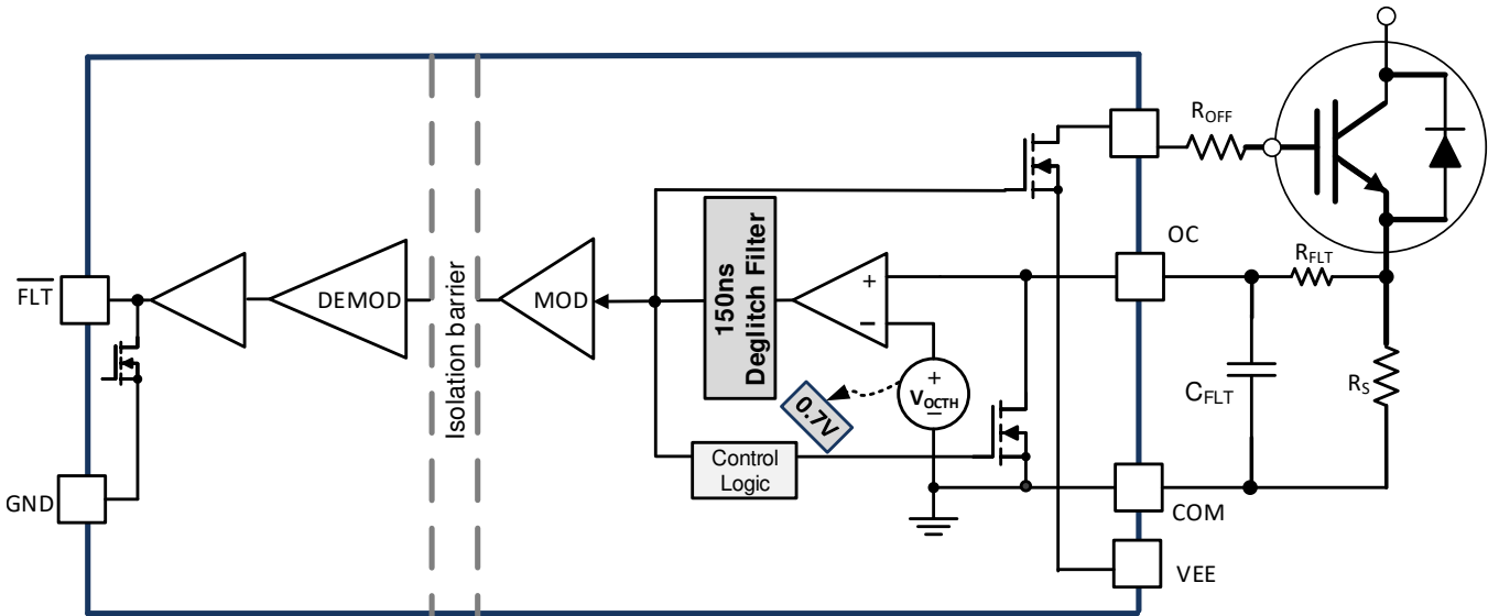
Figure 52. Overcurrent and Short Circuit Protection Based on Shunt Resistor
