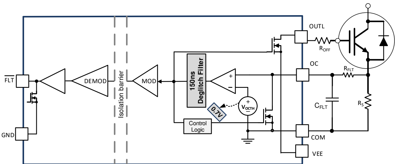
Figure 41. Overcurrent and Short Circuit Protection
