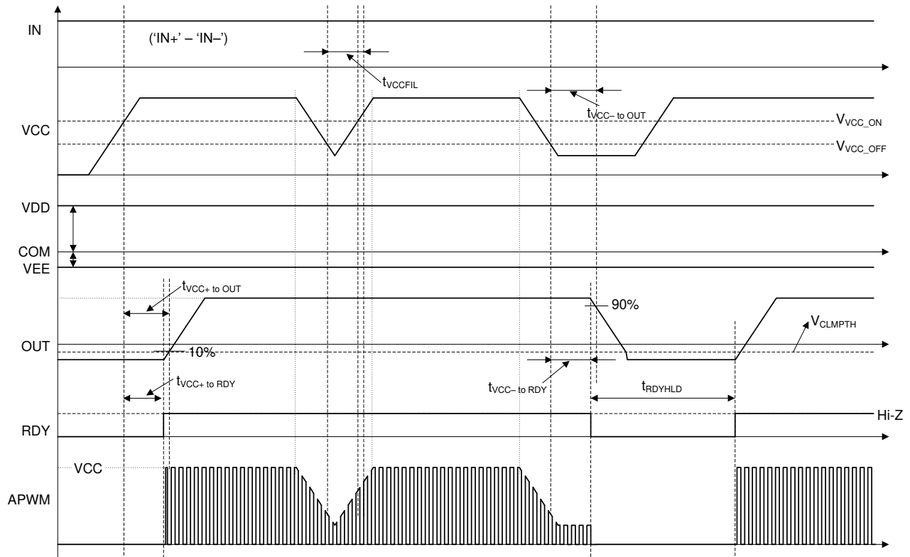
Figure 34. VCC UVLO Protection Timing Diagram
