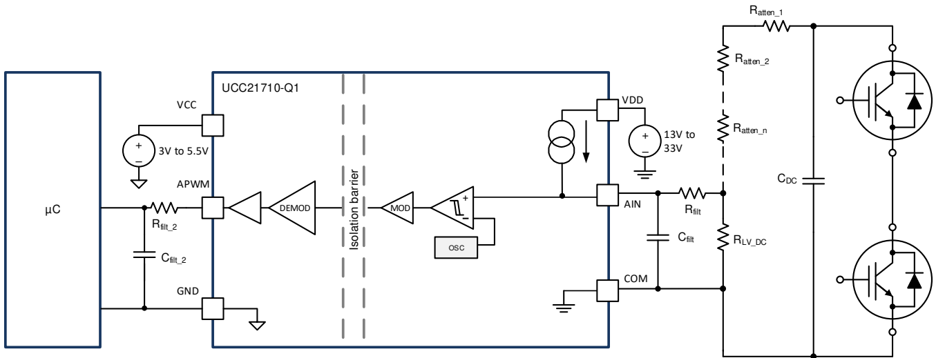
Figure 58. DC-link Voltage Sensing Configuration
