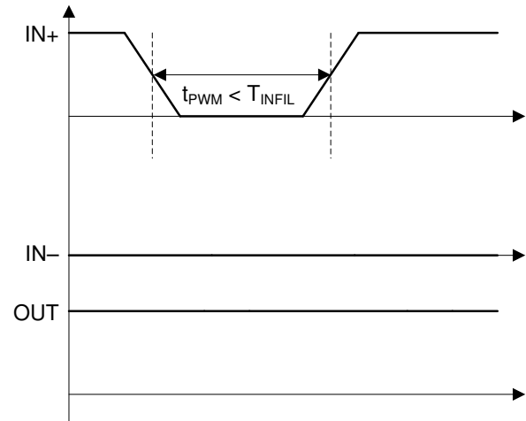
Figure 30. IN+ OFF Deglitch Filter
