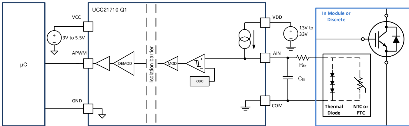
Figure 43. Isolated Analog to PWM Signal
