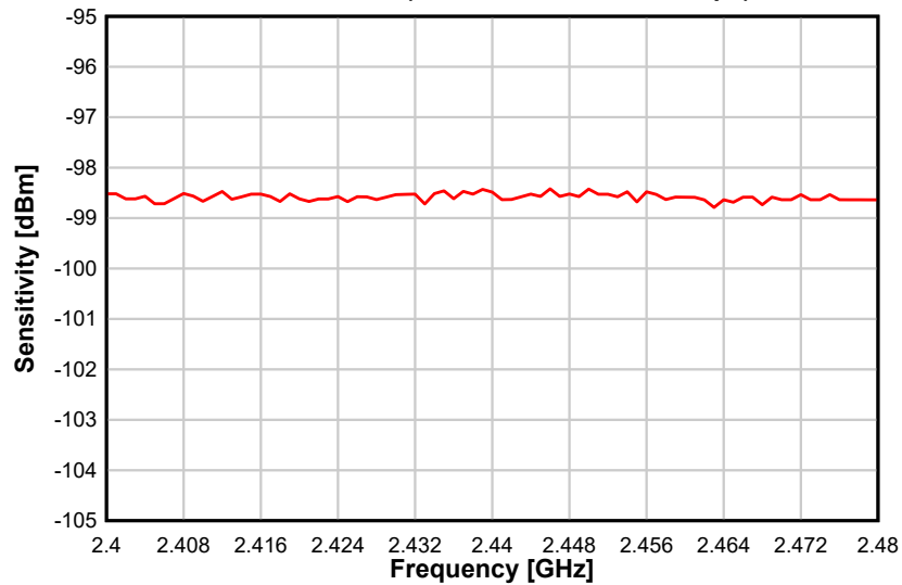
Figure 8-11. Sensitivity vs. Frequency (250 kbps, 2.44 GHz)
