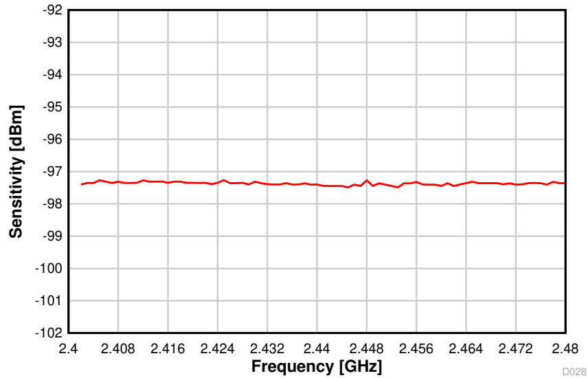
Figure 8-10. Sensitivity vs. Frequency (BLE 1 Mbps, 2.44 GHz)
