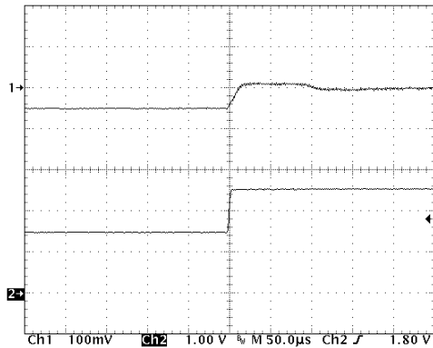
( V_{IN} = 1.5 \text{ V to } 2.5 \text{ V} ; L = 5.6 \mu\text{H} , C_{OUT} = 22 \mu\text{F} , I_{LOAD} = 100 \text{ mA} ) Upper Trace: Output Voltage Ripple, 100 mV/Division Lower Trace: Battery Voltage, V_{IN} , 1.0 V/Division
