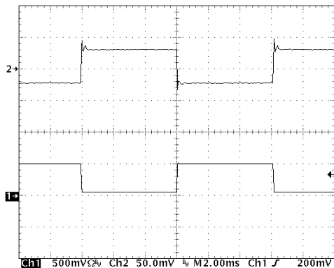
( V_{OUT} = 3.3 \text{ V} , I_{LOAD} = 50 \text{ mA to } 500 \text{ mA} ; L = 5.6 \mu\text{H} , C_{OUT} = 22 \mu\text{F} ) Upper Trace: Output Voltage Ripple, 50 mV/Division Lower Trace: Load Current, I_{LOAD} , 500 mA/Division
