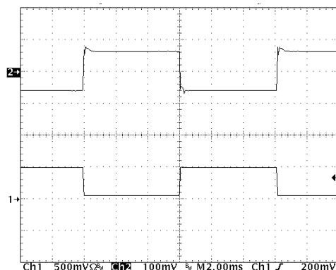
( V_{OUT} = 5.0 \text{ V} , I_{LOAD} = 50 \text{ mA to } 500 \text{ mA} ; L = 5.6 \mu\text{H} , C_{OUT} = 22 \mu\text{F} ) Upper Trace: Output Voltage Ripple, 100 mV/Division Lower Trace: Load Current, I_{LOAD} , 500 mA/Division
