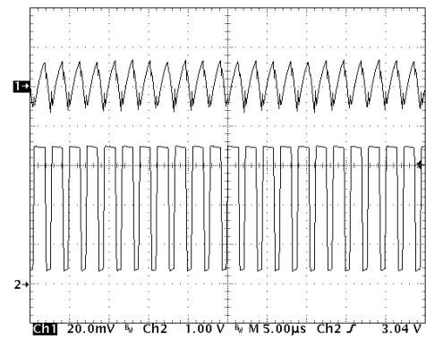
( V_{IN} = 2.5 \text{ V} , V_{OUT} = 3.3 \text{ V} , I_{LOAD} = 500 \text{ mA} ; L = 5.6 \mu\text{H} , C_{OUT} = 22 \mu\text{F} ) Upper Trace: Output Voltage Ripple, 20 mV/Division Lower Trace: Voltage at LX pin, 1.0 V/Division
