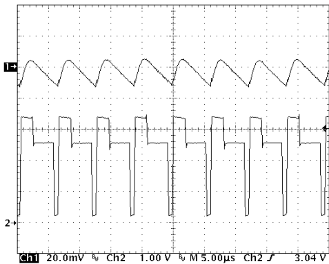
( V_{IN} = 2.5 \text{ V} , V_{OUT} = 3.3 \text{ V} , I_{LOAD} = 50 \text{ mA} ; L = 5.6 \mu\text{H} , C_{OUT} = 22 \mu\text{F} ) Upper Trace: Output Voltage Ripple, 20 mV/Division Lower Trace: Voltage at Lx pin, 1.0 V/Division
