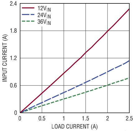
Input vs Load Current V_{OUT} = 10V
