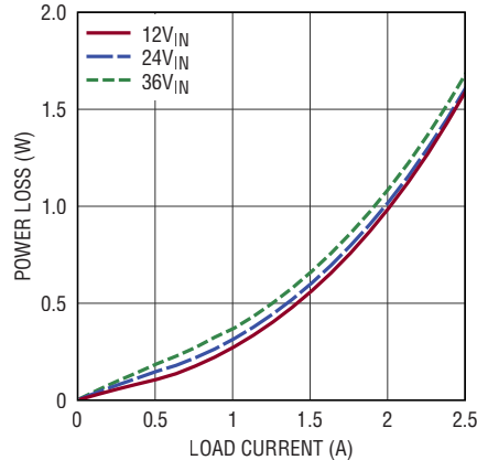
Power Loss, V_{OUT} = 1.2V BIAS = 5V, Burst Mode Operation
