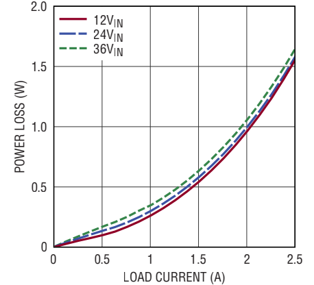
Power Loss, V_{OUT} = 1V BIAS = 5V, Burst Mode Operation
