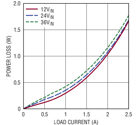
Power Loss, V_{OUT} = 1.8V BIAS = 5V, Burst Mode Operation
