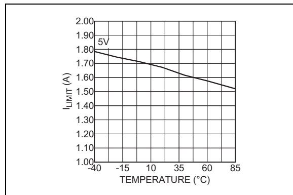
FIGURE 2-6: I LIMIT vs. Temperature (MIC20XX-1.2).
