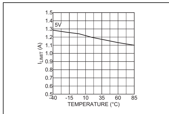
FIGURE 2-5: I LIMIT vs. Temperature (MIC20XX-0.8).
