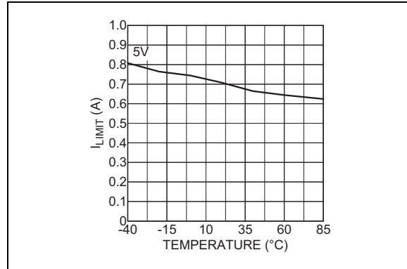
FIGURE 2-4: I LIMIT vs. Temperature (MIC20XX-0.5).
