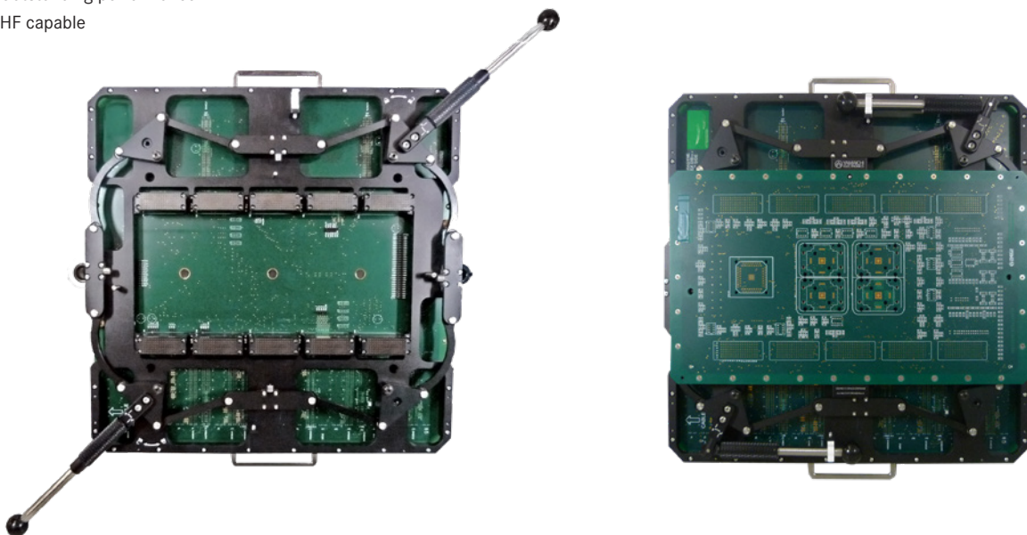
Universal Interface Board with Locking Mechanism, open position (no DUT)
