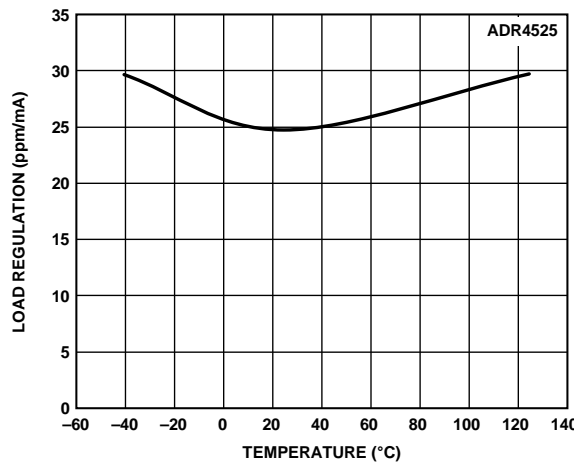
Figure 23. ADR4525 Load Regulation vs. Temperature (Sourcing)
