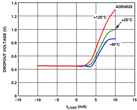
Figure 22. ADR4525 Dropout Voltage vs. Load Current
