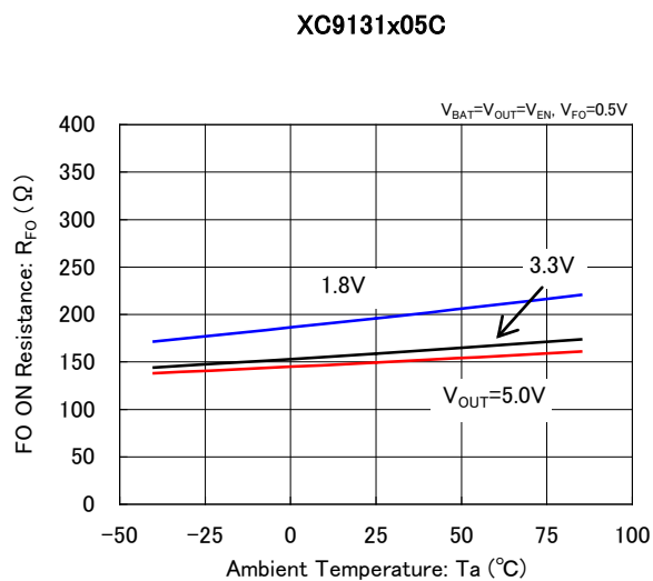
(20) FO ON Resistance vs. Ambient Temperature
