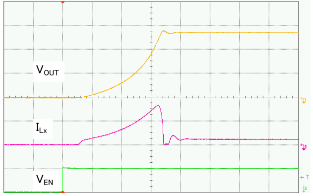
XC9131x05C (1.2MHz) V_{OUT}:2V/div , I_{Lx}:500mA/div , V_{EN}:5V/div , Time:100us/div L=4.7\mu H (LTF5022-LC), C_L=20\mu F (LMK212BJ106KG*2) C_{IN}=10\mu F (LMK212BJ106KG), C_{OD}=0.47\mu F (EMK107BJ474KA) R_{FB1}=270k\Omega , R_{FB2}=30k\Omega , C_{FB}=10pF
