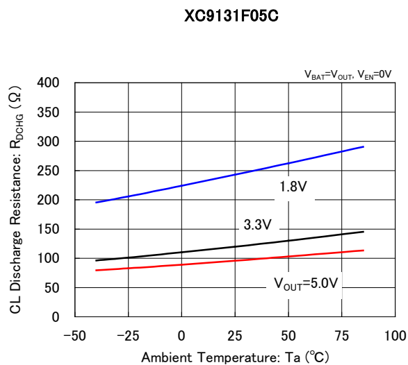
(21) CL Discharge Resistance vs. Ambient Temperature
