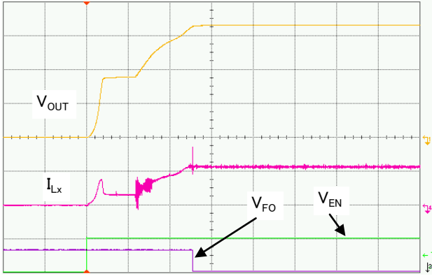
XC9131x05C (1.2MHz) V_{OUT}:1V/div , I_{Lx}:200mA/div , V_{EN}:5V/div , V_{FO}:5V/div Time:2ms/div L=4.7\mu H (LTF5022-LC), C_L=20\mu F (LMK212BJ106KG*2) C_{IN}=10\mu F (LMK212BJ106KG), C_{OD}=0.47\mu F (EMK107BJ474KA) R_{FB1}=560k\Omega , R_{FB2}=100k\Omega , C_{FB}=10pF
