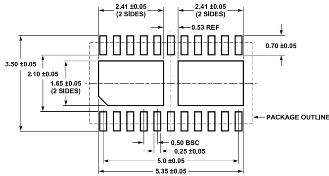
Figure 132. 22-Lead, 6 mm × 3 mm, Plastic DFN (05-08-7071) Dimensions shown in millimeters
