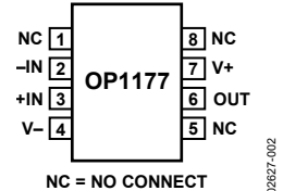
Figure 2. 8-Lead SOIC_N (R Suffix)
