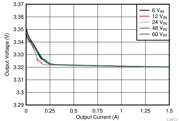
V_{OUT} = 3.3\text{ V} 400 kHz Figure 10-7. Load Regulation
