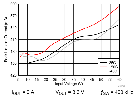
Figure 8-6. I_{PEAK-MIN}
