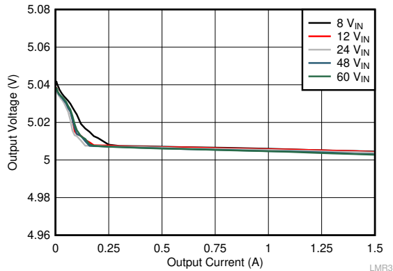
V_{OUT} = 5\text{ V} 400 kHz Figure 10-6. Load Regulation
