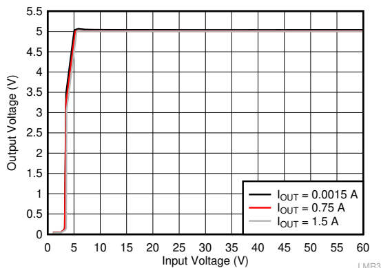
V_{OUT} = 5\text{ V} 400 kHz Figure 10-8. Line Regulation
