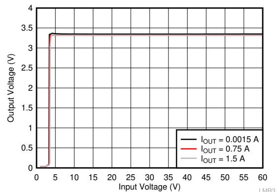
V_{OUT} = 3.3\text{ V} 400 kHz Figure 10-9. Line Regulation
