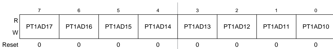
Figure 24-61. Port AD1 Data Register 1 (PT1AD1)
