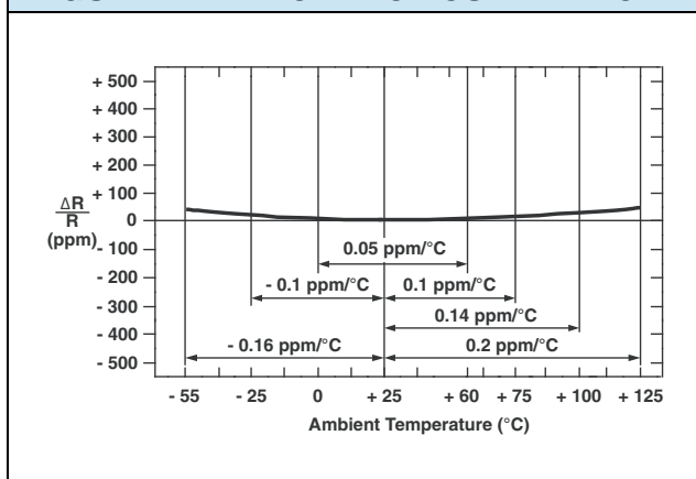
FIGURE 4 - TYPICAL TCR CURVE Z-FOIL
