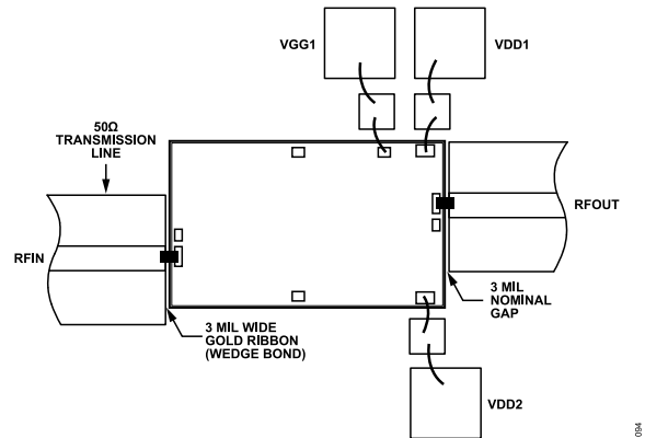
Figure 94. Assembly Diagram
