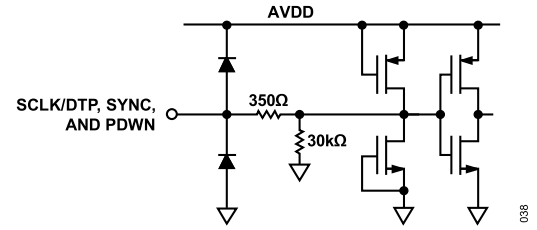
Figure 39. Equivalent SCLK/DTP, SYNC, and PDWN Input Circuit
