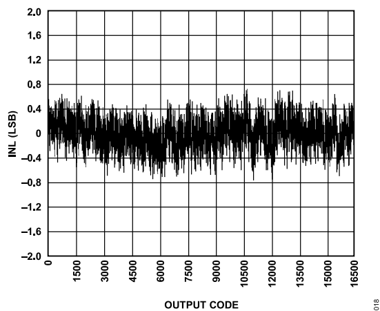
Figure 19. INL, f_{\text{IN}} = 9.7 \text{ MHz} , f_{\text{SAMPLE}} = 65 \text{ MSPS}
