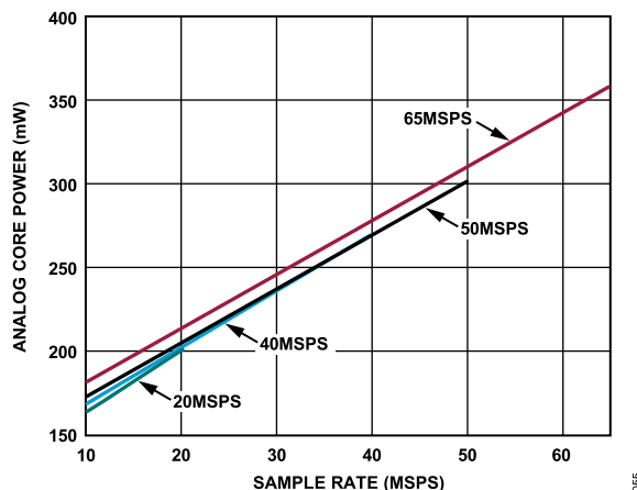
Figure 56. Analog Core Power vs. f_{\text{SAMPLE}} for f_{\text{IN}} = 9.7 \text{ MHz}
