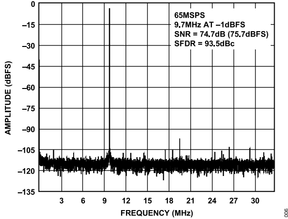
Figure 6. Single-Tone 16k FFT with f_{IN} = 9.7 \text{ MHz} , f_{SAMPLE} = 65 \text{ MSPS}
