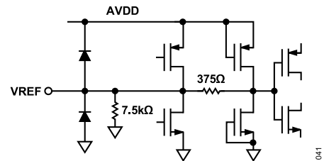
Figure 42. Equivalent VREF Circuit
