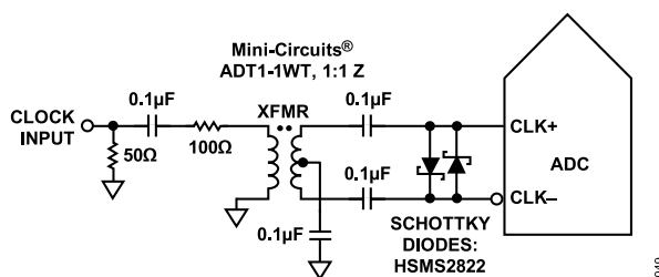
Figure 50. Transformer-Coupled Differential Clock (Up to 200 MHz)
