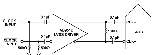
Figure 53. Differential LVDS Sample Clock (Up to 520 MHz)
