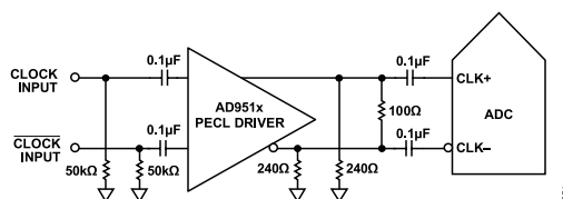
Figure 52. Differential PECL Sample Clock (Up to 520 MHz)
