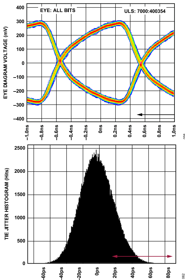
Figure 59. Data Eye for LVDS Outputs in ANSI-644 Mode with Trace Lengths Less Than 24 Inches on Standard FR-4, External 100 Ω Far Termination Only
