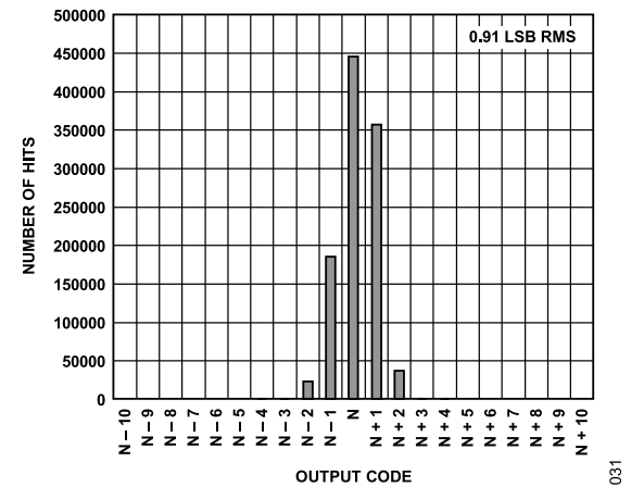
Figure 32. Input-Referred Noise Histogram, f_{SAMPLE} = 40 MSPS
