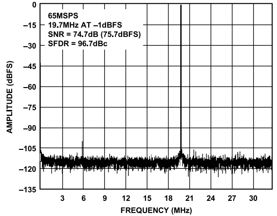
Figure 9. Single-Tone 16k FFT with f_{IN} = 19.7 \text{ MHz} , f_{SAMPLE} = 65 \text{ MSPS} , CLK Divider = 8
