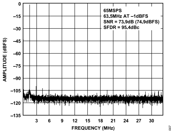
Figure 7. Single-Tone 16k FFT with f_{IN} = 63.5 \text{ MHz} , f_{SAMPLE} = 65 \text{ MSPS} , CLK Divider = 8
