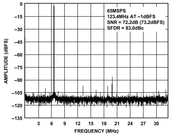
Figure 11. Single-Tone 16k FFT with f_{IN} = 123.4 \text{ MHz} , f_{SAMPLE} = 65 \text{ MSPS} , CLK Divider = 8
