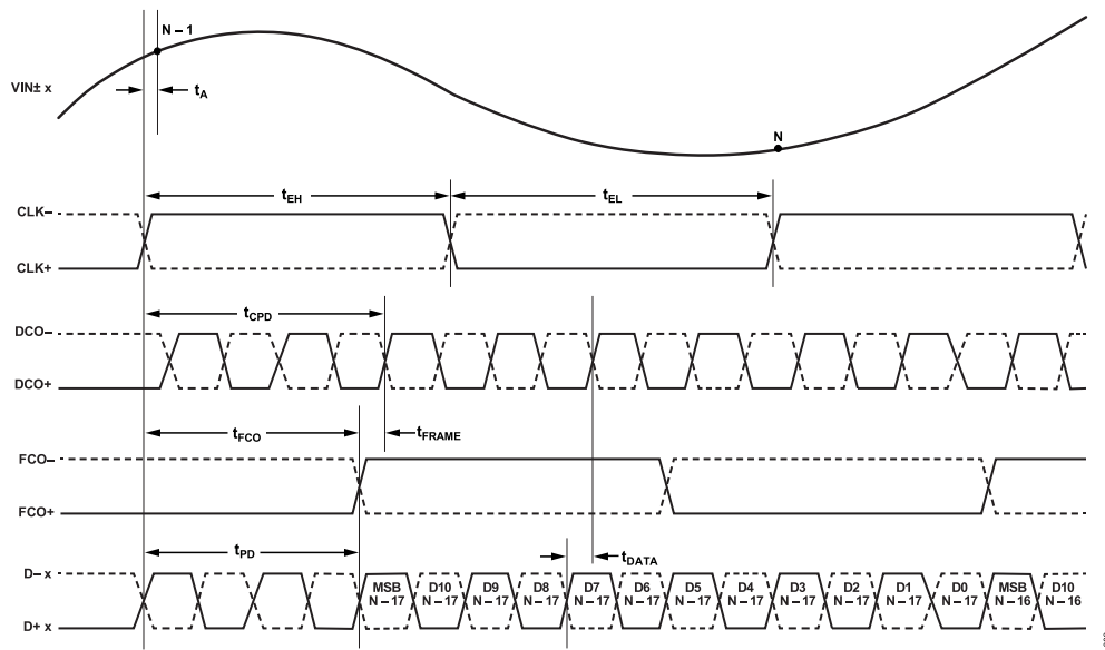
Figure 3. Word-Wise DDR, 1x Frame, 12-Bit Output Mode
