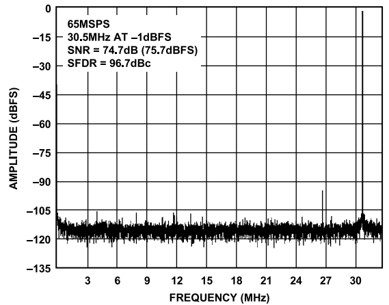
Figure 10. Single-Tone 16k FFT with f_{IN} = 30.5 \text{ MHz} , f_{SAMPLE} = 65 \text{ MSPS} , CLK Divider = 8
