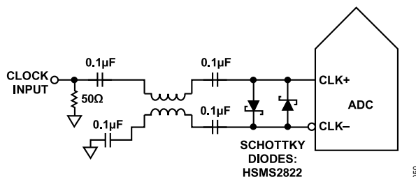
Figure 51. Balun-Coupled Differential Clock (65 MHz to 520 MHz)
