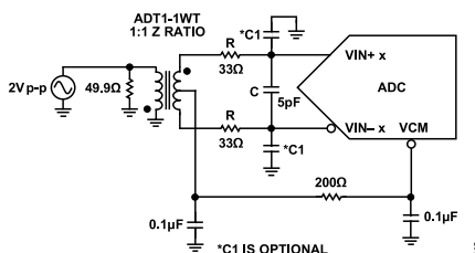
Figure 47. Differential Transformer-Coupled Configuration for Baseband Applications
