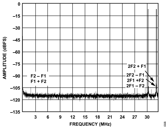
Figure 8. Two-Tone 16k FFT with f_{IN1} = 30 \text{ MHz} and f_{IN2} = 32 \text{ MHz} , f_{SAMPLE} = 65 \text{ MSPS}
