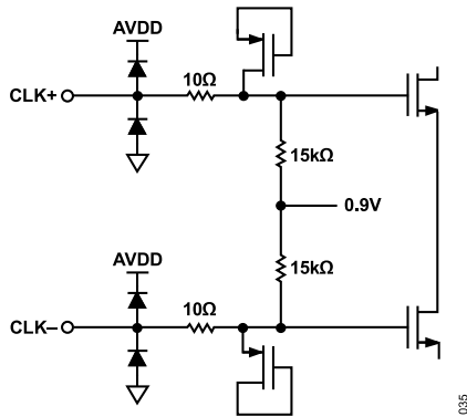
Figure 36. Equivalent Clock Input Circuit
