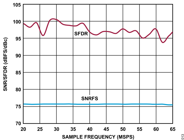
Figure 14. SNR/SFDR vs. Encode, f_{IN} = 19.7 MHz, CLK Divider = 4
