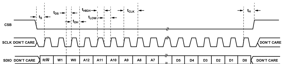
Figure 61. Serial Port Interface Timing Diagram
