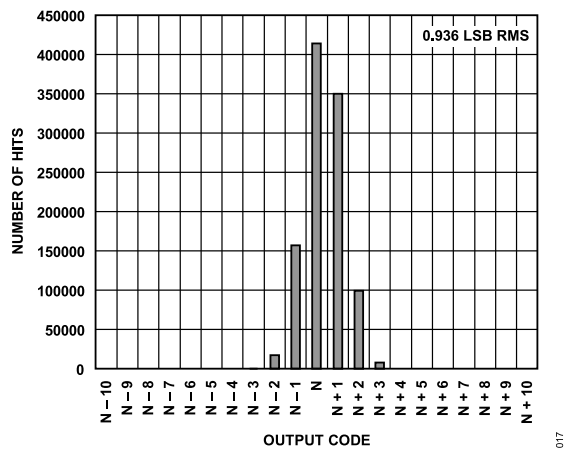
Figure 18. Input-Referred Noise Histogram, f_{\text{SAMPLE}} = 65 \text{ MSPS}
