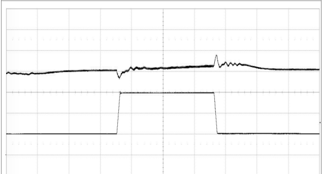
Output voltage response to load current Top trace: output voltage (100 mV/div.). Step-change (10-30-10 A) at: Bottom trace: load current (10 A/div.). T_{P1} = +25^\circ C , V_I = 12 V , V_O = 1.0 V Time scale: (0.1 ms/div.). di/dt = 2 A/\mu s , f_{sw} = 320 kHz C_O = 4000 \mu F
