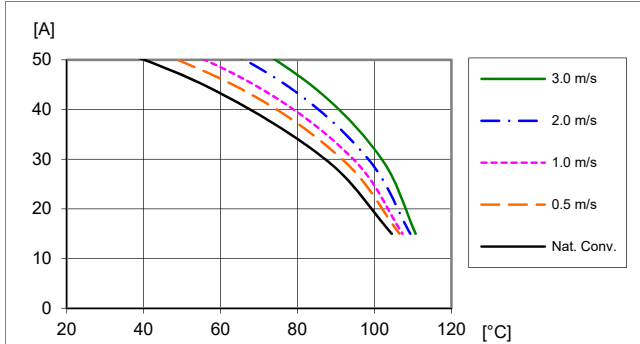
Output Current Derating, V_o = 1.0 V
