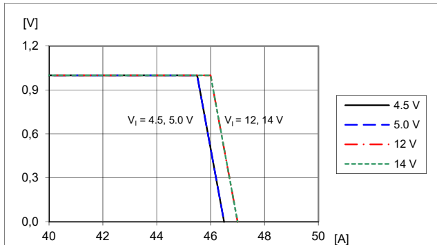
Current Limit Characteristics, V_O = 1.0 V
