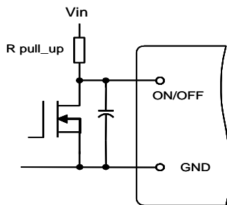
Fig. 14 Circuit for Negative Logic Control
