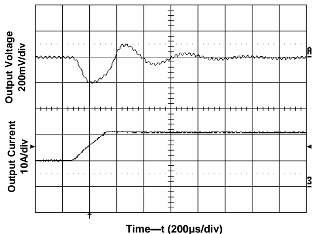
Figure 9. Transient Load Response Input voltage 12V, Output current 10A -> 20A, Slew rate 0.5A/μs
