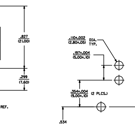
RECOMMENDED P.C. BOARD PLATED-THRU HOLE LAYOUT (4 CKT. SHOWN FOR REF.)
