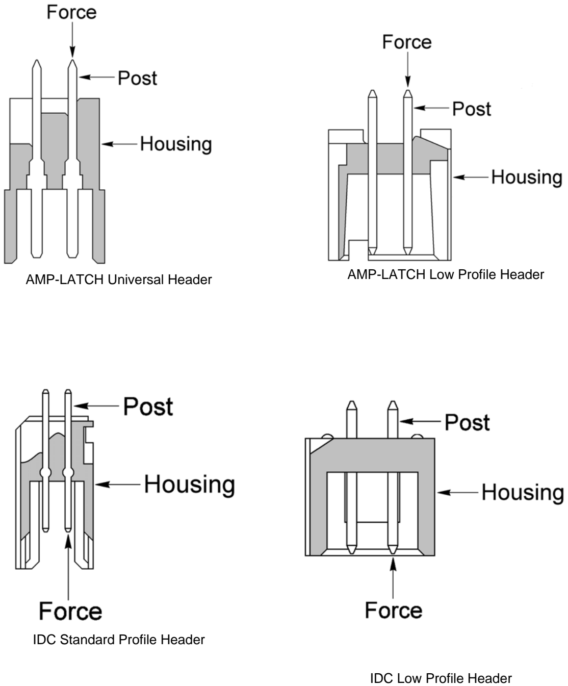
Figure 3 Contact Retention
