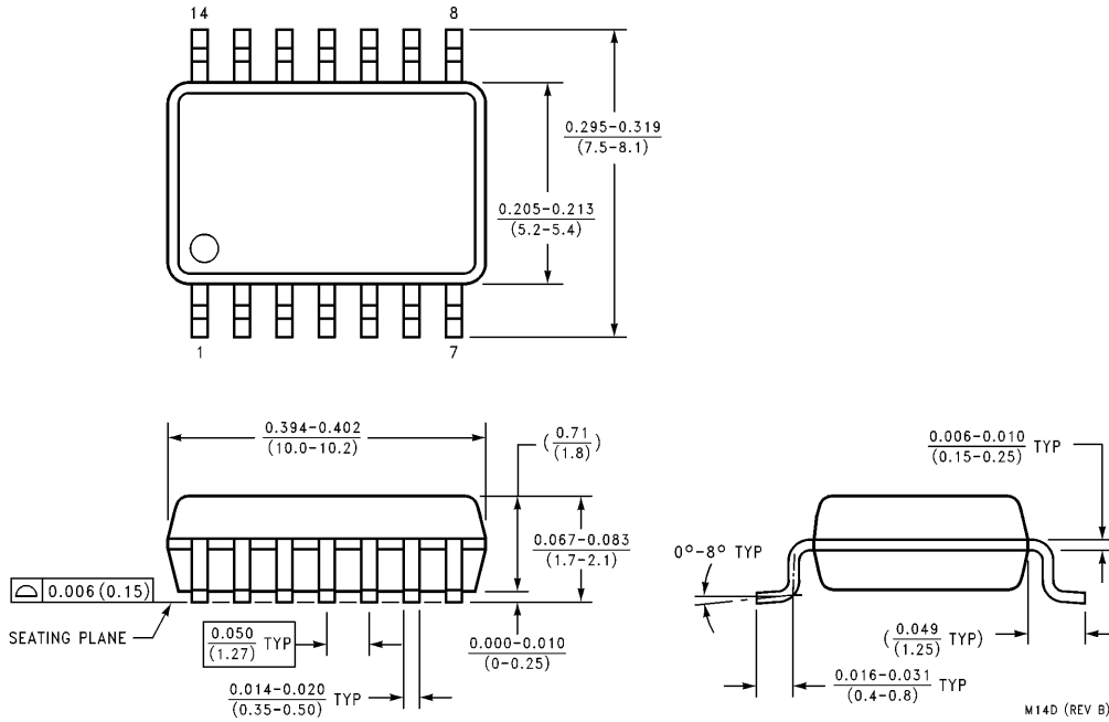
14-Lead (0.300" Wide) Molded Small Outline Package, EIAJ (SJ) Order Number 74LVQ04SJ or 74LVQ04SJX NS Package Number M14D
