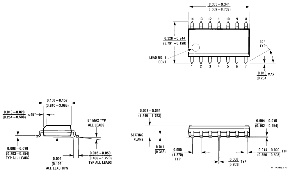
14-Lead Small Outline Integrated Circuit (S) Order Number 74LVQ04SC or 74LVQ04SCX NS Package Number M14A
