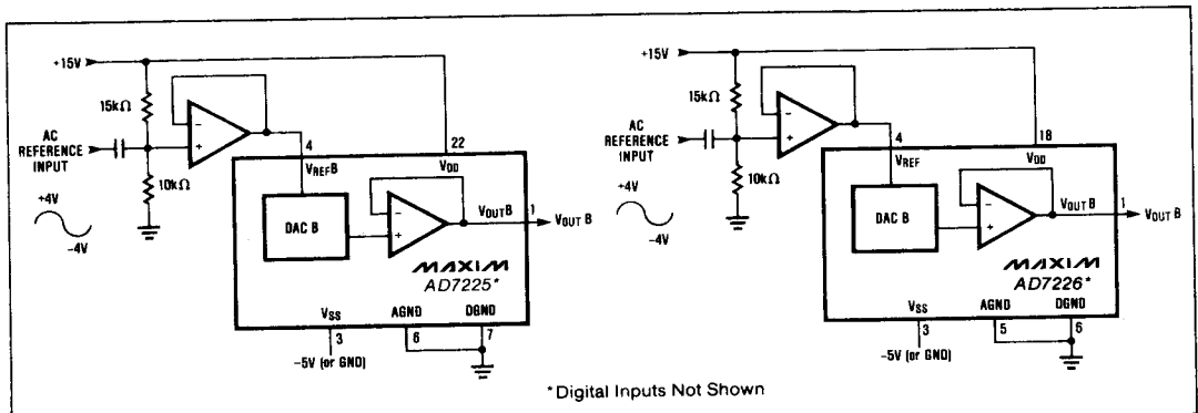
Figure 13. AC Reference Input Circuit
