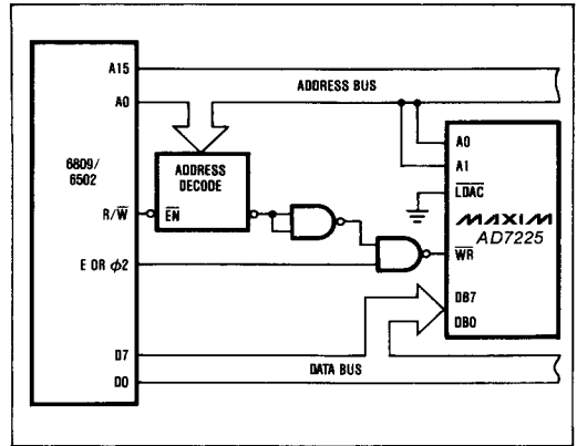
Figure 16. AD7225 to 6089/6502 Interface, Single-Buffered Mode
