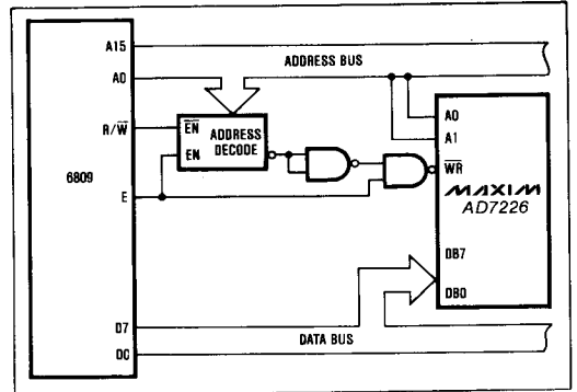
Figure 20. AD7226 to 6809 Interface
