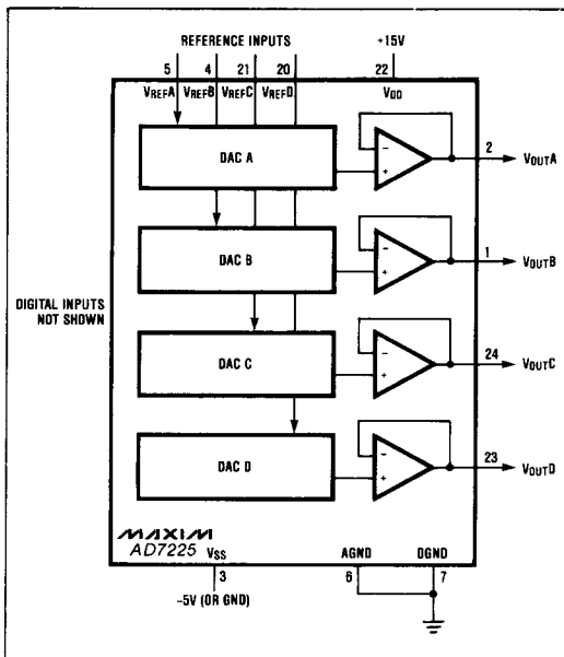
Figure 9. AD7225 Unipolar Output Circuit
