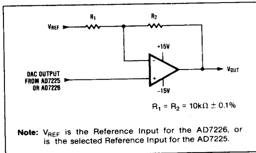
Figure 11. Bipolar Output Circuit
