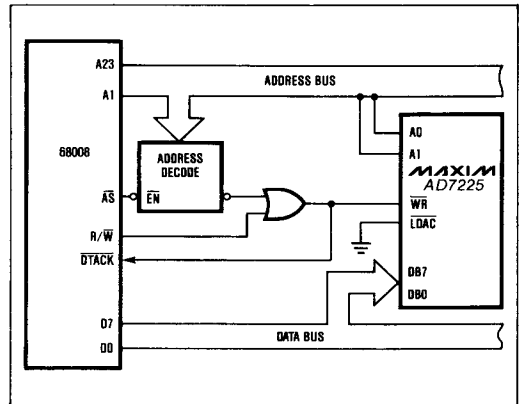
Figure 18. AD7225 to 68008 Interface, Single-Buffered Mode
