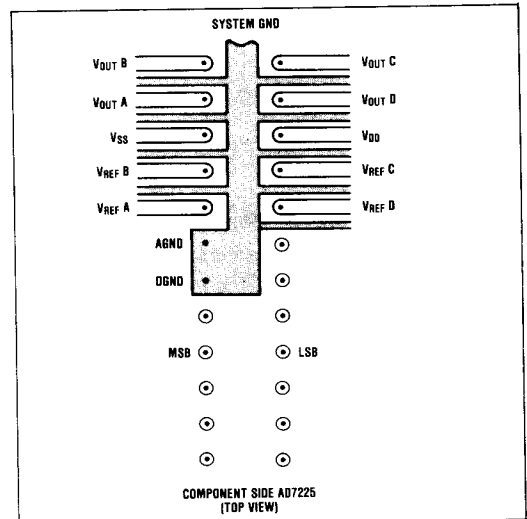
Figure 8. Suggested AD7225 PCB Layout for Minimizing Crosstalk
