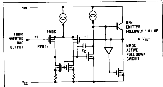
Figure 4. Simplified Output Buffer Circuit
