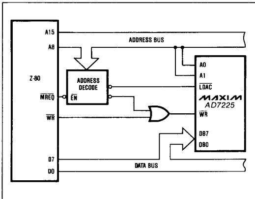
Figure 17. AD7225 to Z-80 Interface Double-Buffered Mode
