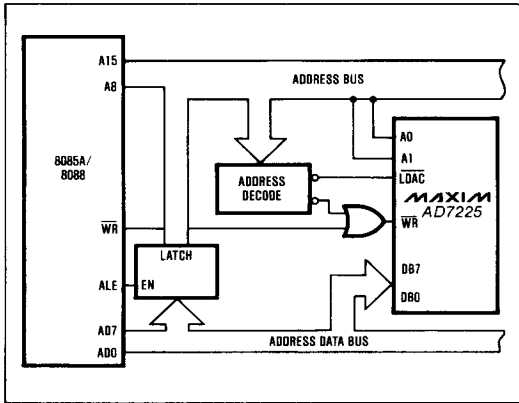
Figure 15. AD7225 to 8085A/8088 Interface, Double-Buffered Mode
