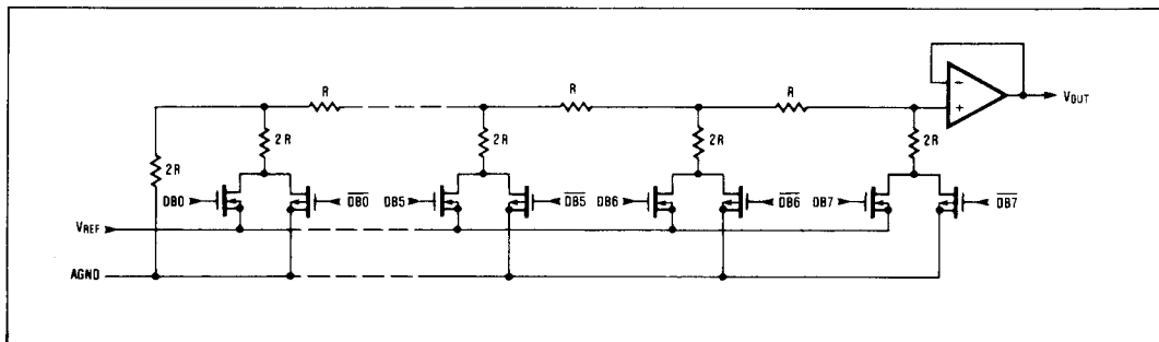
Figure 1. Simplified DAC Circuit Diagram
