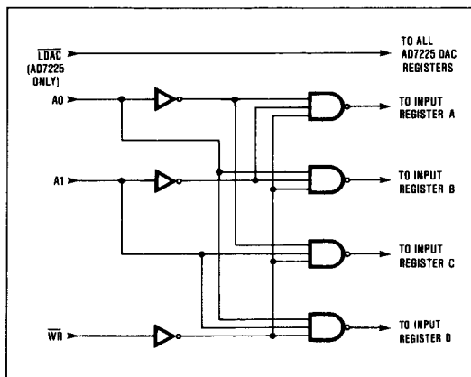
Figure 5. AD7225, AD7226 Input Control Logic
