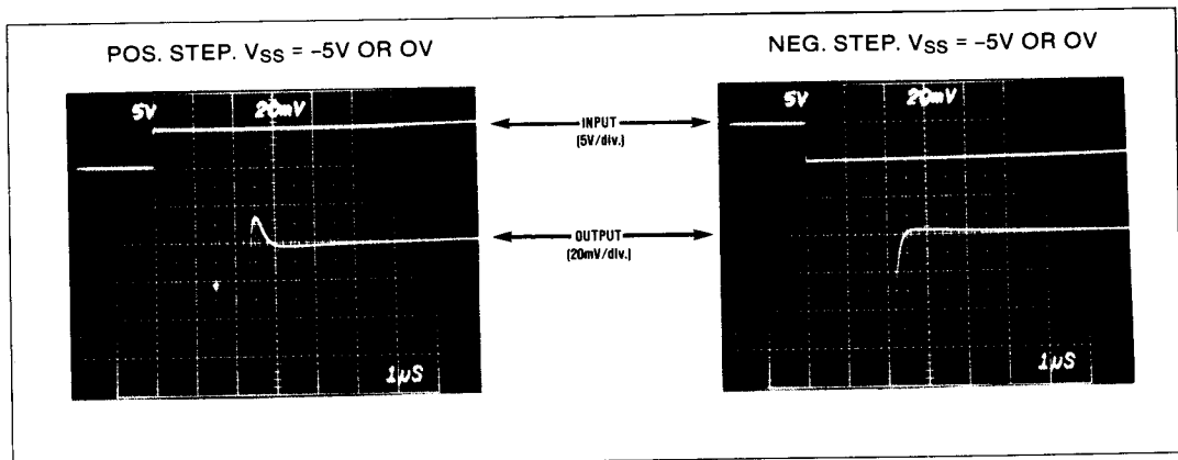
Figure 2. Positive and Negative Settling Times, V_{SS} = 0V or -5V
