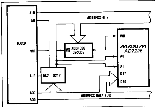
Figure 19. AD7226 to 8085A Interface
