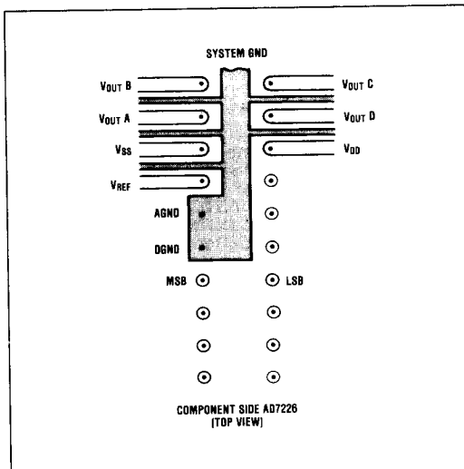
Figure 7. Suggested AD7226 PCB Layout for Minimizing Crosstalk
