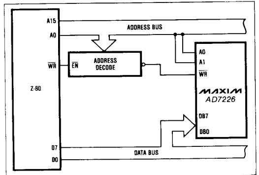
Figure 22. AD7226 to Z-80 Interface
