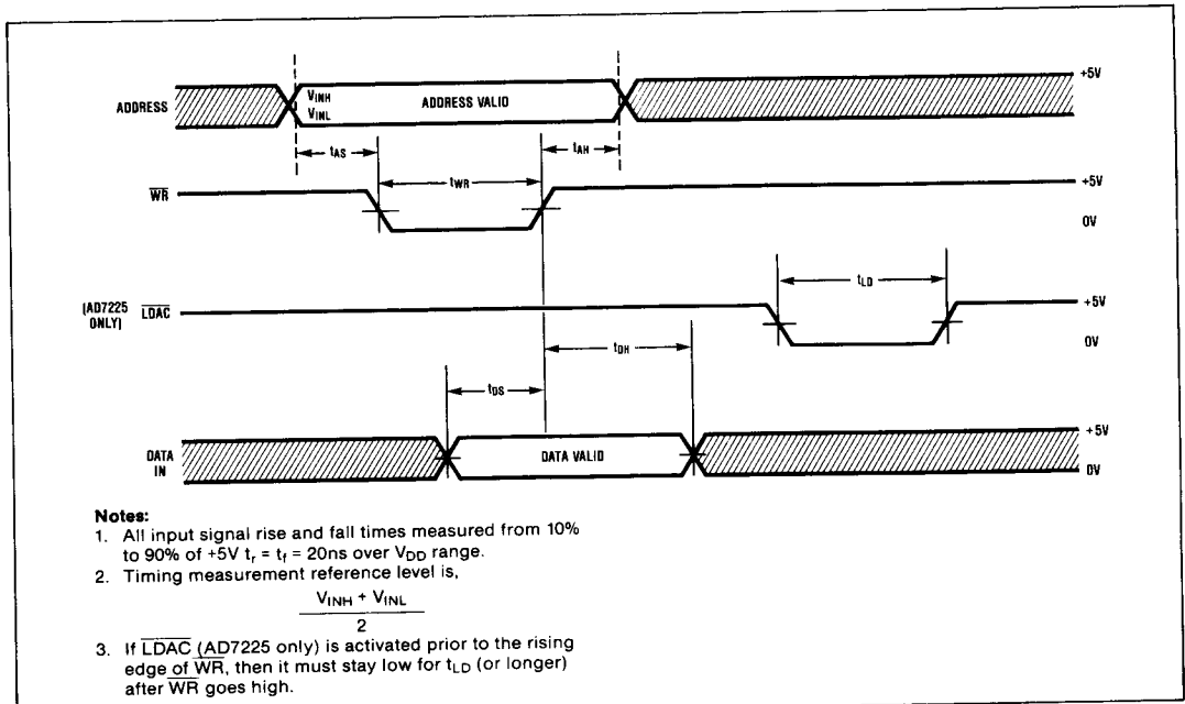
Figure 6. Write Cycle Timing Diagram
