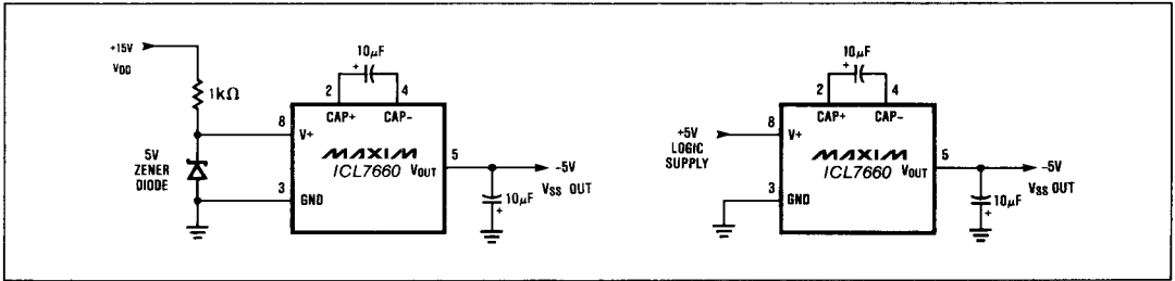
Figure 14. Generating -5V for V SS
