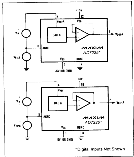
Figure 12. AGND Bias Circuits
