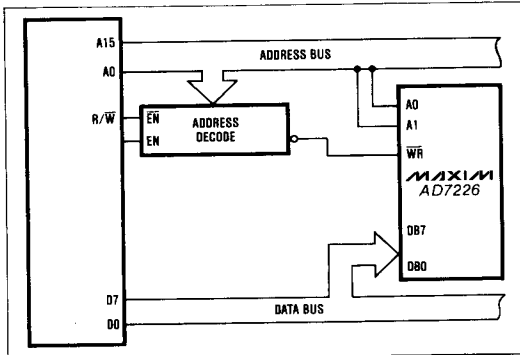
Figure 21. AD7226 to 6502 Interface
