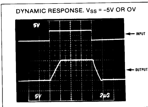
Figure 3. Dynamic Response, V_{SS} = 0V or -5V
