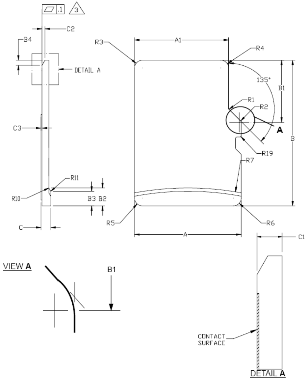
Figure 42-12: Dimensions Of microSD (Top View)
