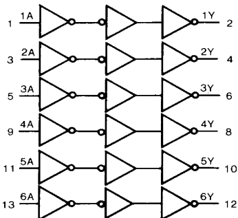
Fig. 1 Logic diagram
