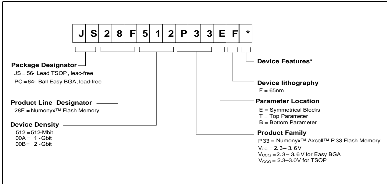
Figure 29: Decoder for P33-65nm Products
