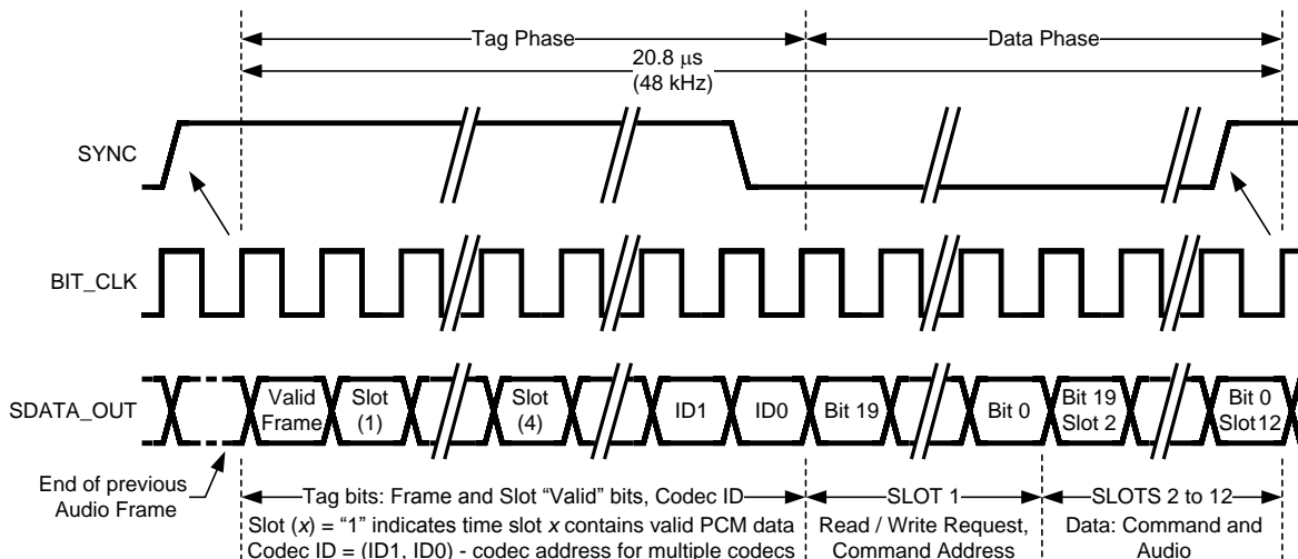
Figure 18. AC Link Output Frame
