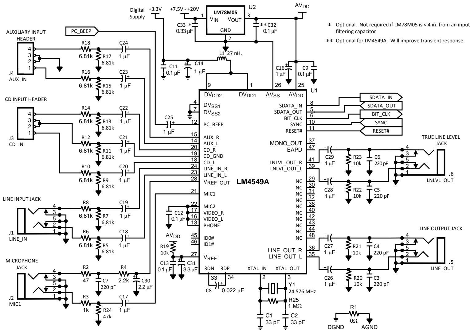
Figure 10. LM4549A Reference Design, Typical Application, Single Codec, 1 Vrms and 2 Vrms inputs, EMC output filters
