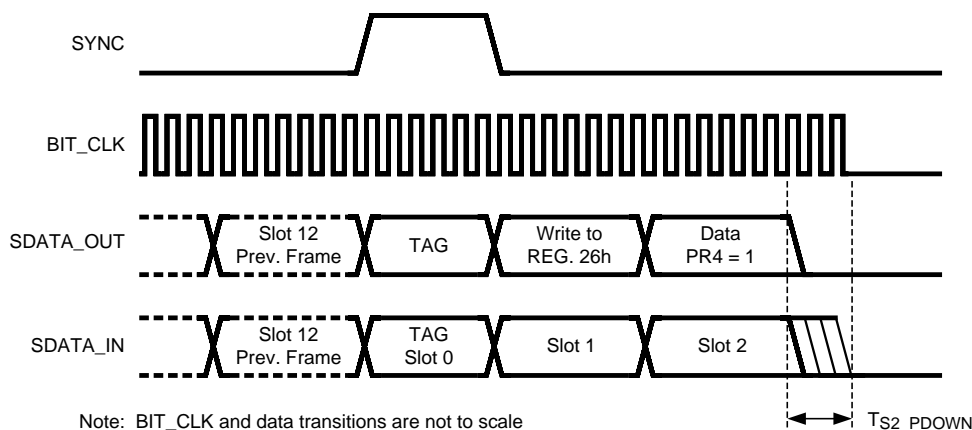
Figure 22. AC Link Powerdown Timing
