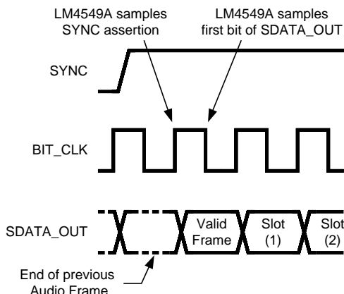
Figure 19. Start of AC Link Output Frame
