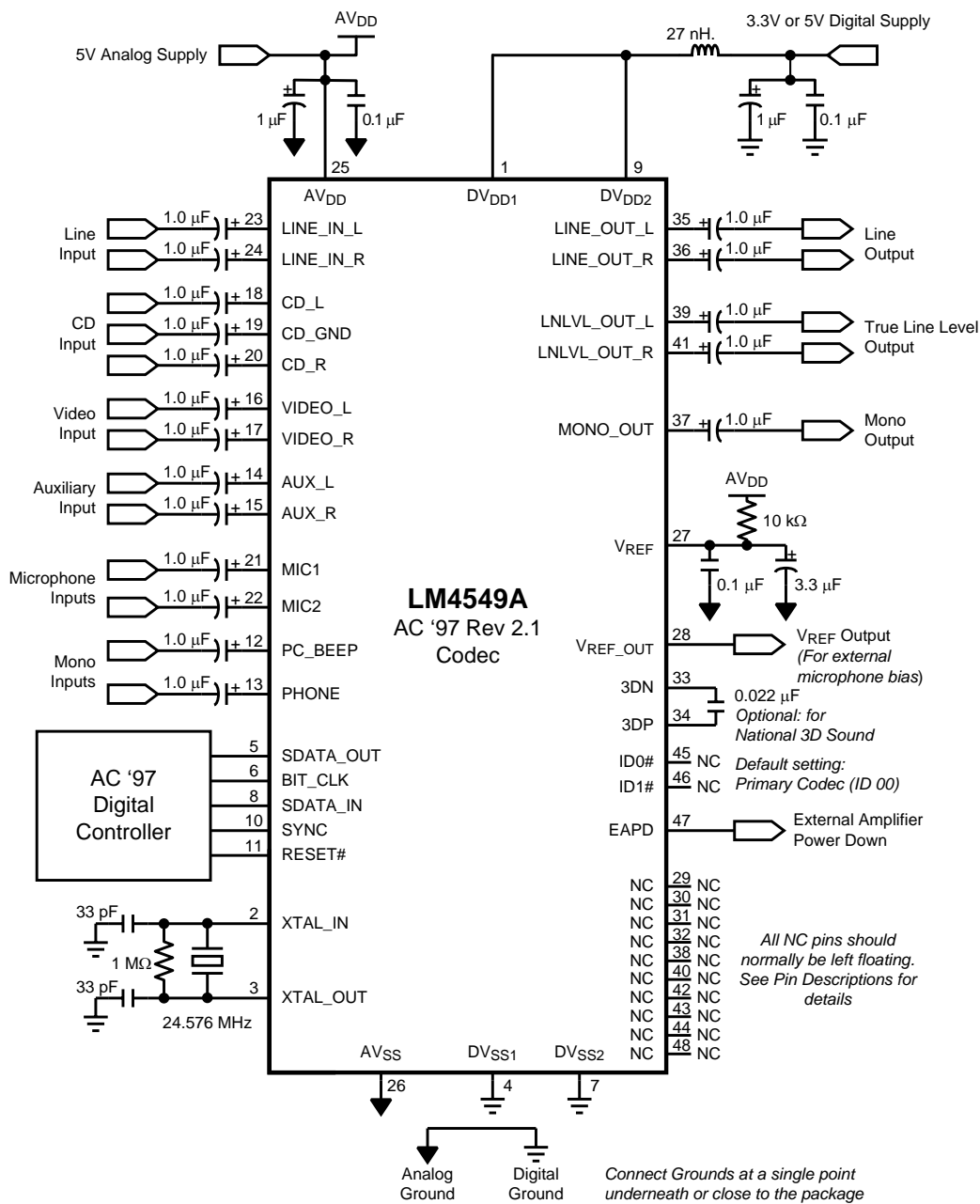
Figure 9. LM4549A Typical Application Circuit, Single Codec, 1 Vrms inputs
