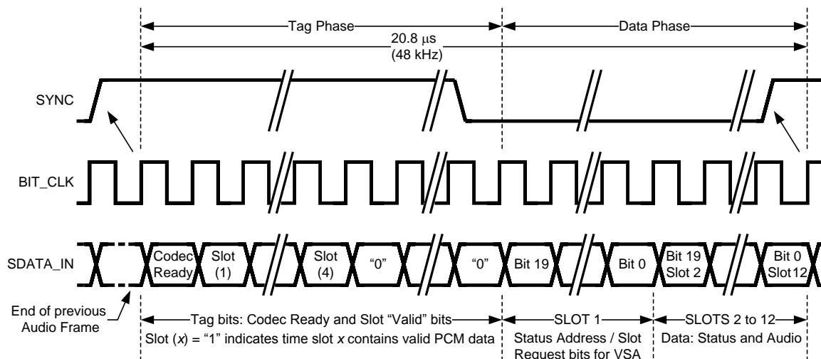
Figure 20. AC Link Input Frame
