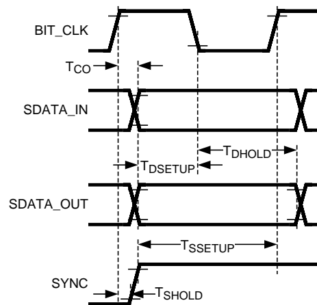
Figure 3. Data Delay, Setup and Hold
