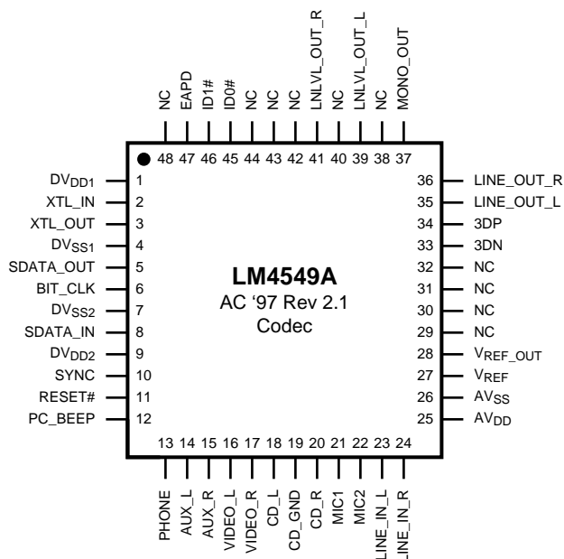
48 Pin LQFP - Top View See Package Number PT
