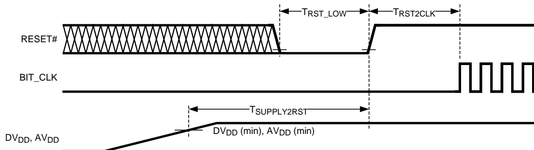
Figure 6. Power On Reset
