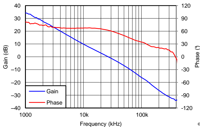
Figure 11. V OUT = 1.8 V, I OUT = 4 A, C OUT = 200 μF ceramic, f SW = 500 kHz
