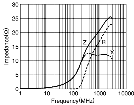
MMZ1608D500C
