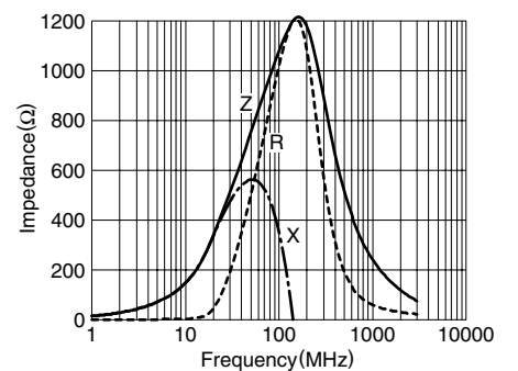
MMZ1608Y102B
