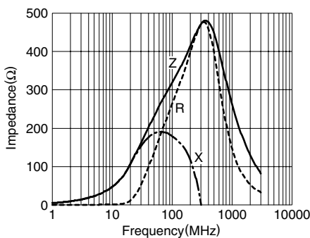
MMZ1608Y301B
