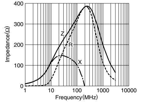
MMZ1608Y150B
