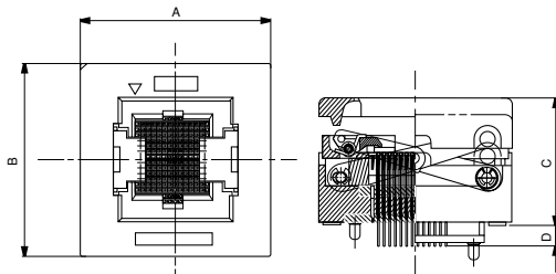
OTB-144-0.8 Series
