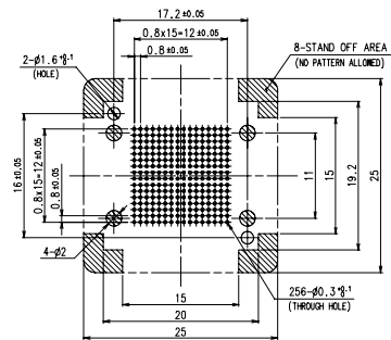
OTB-256-0.8 Series
