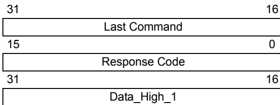
FIGURE 16-2: RESPONSE FORMAT
