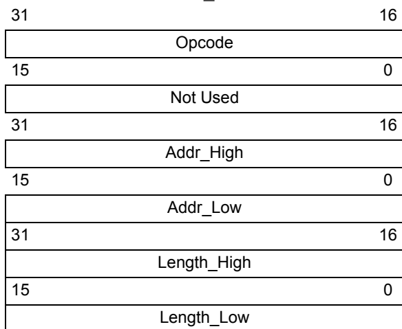
FIGURE 16-20: GET_CRC COMMAND
