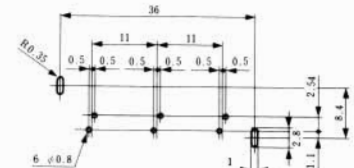
TM2RE-1806( 50 )
